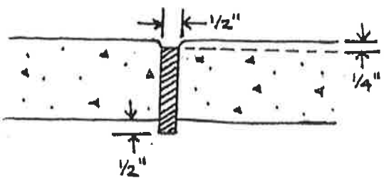
EXPANSION JOINT
